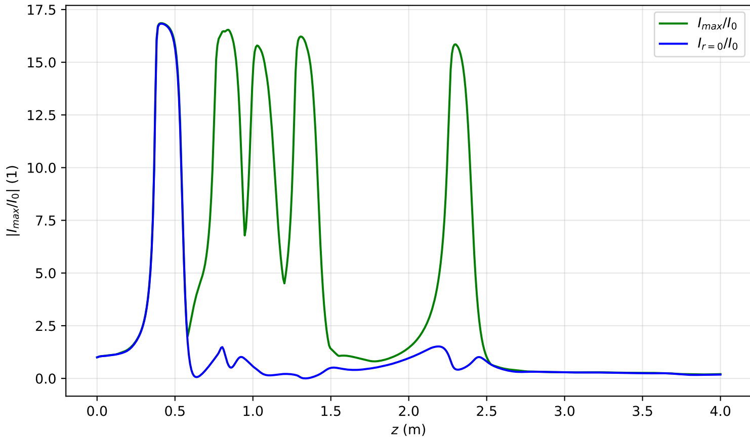
I_{\max}(x=0, y=0, z)/I_0 , \text{Pin}=6.6\text{Pcr} , noisy input, artificial time
